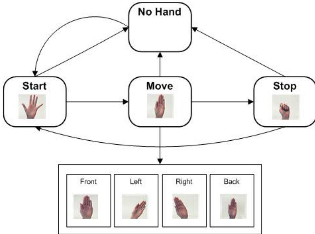
Figure 3: Gesture alphabet and valid gesture transitions.
