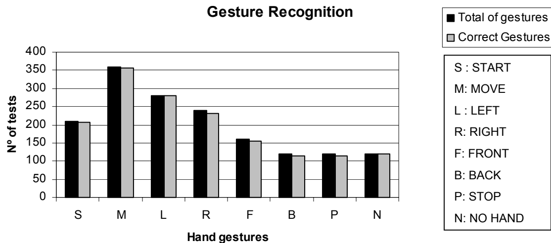
Figure 6: System's performance evaluation results.
