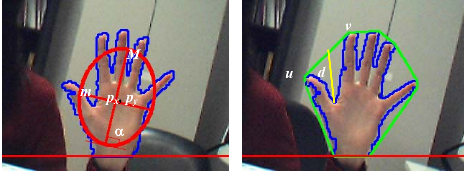
Figure 4: Extracted features for the hand gesture recognition. In the right image, u_i and v_i indicate the start and the end points of the i th-convexity defect, the depth, d_i , is the distance from the farthestmost point of the convexity defect to the convex hull segment.
