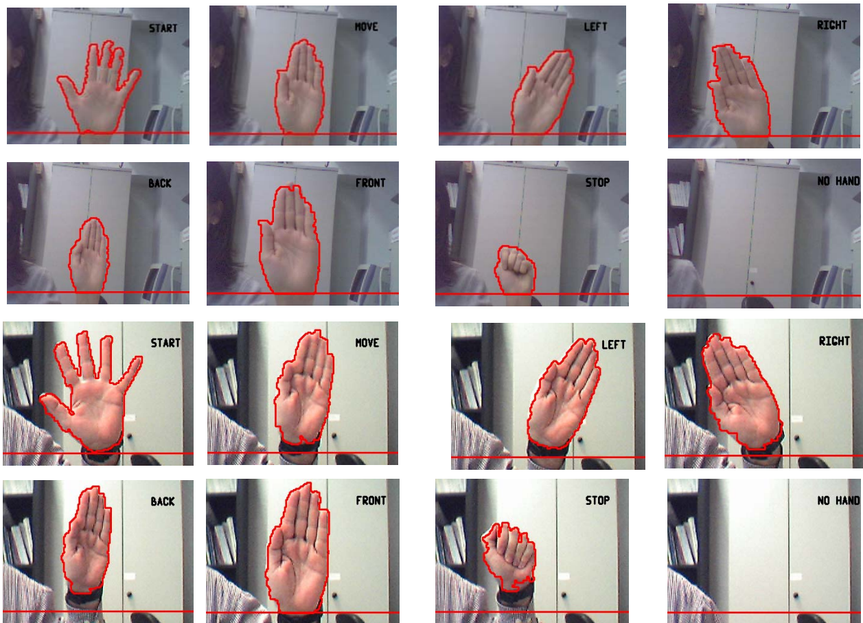
Figure 5: Gesture recognition examples for different lighting conditions, users and hand configurations.
